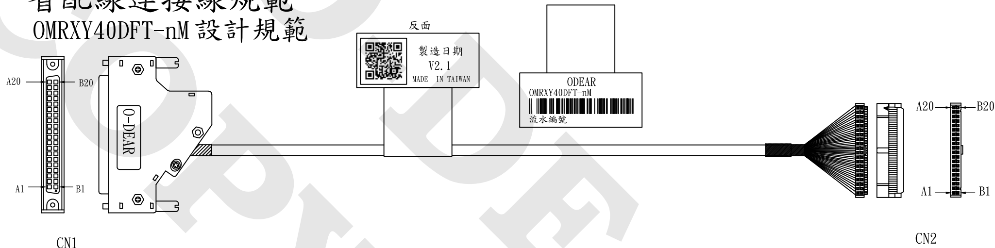
(PLC側) (端子台側)
