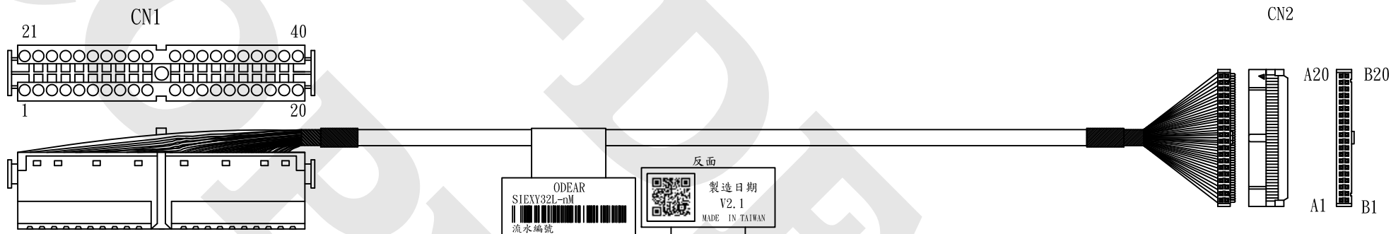
(PLC側) (端子台側) (PLC側) (端子台側)
