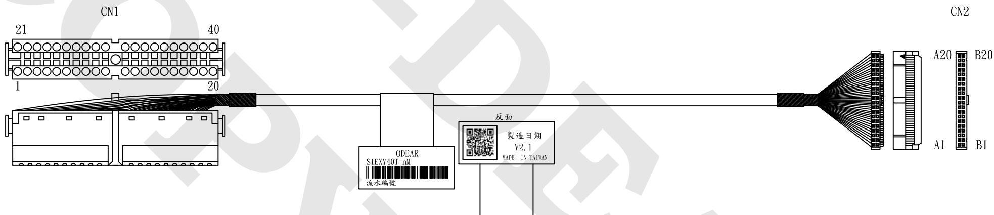
(PLC側) (端子台側)
